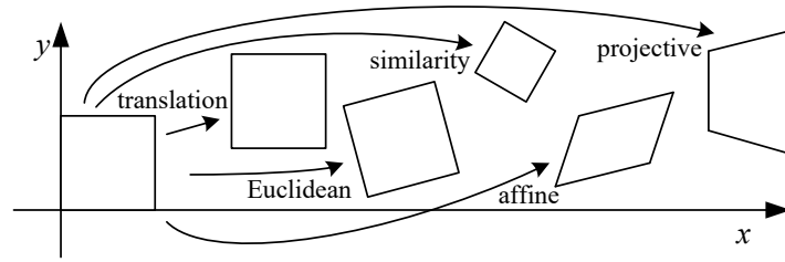
Figure 2.4 Basic set of 2D planar transformations.
