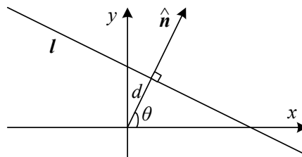
Figure 7.48 2D line equation expressed in terms of the normal \hat{n} and distance to the origin d .
