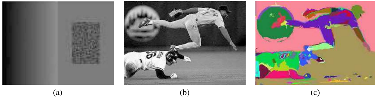
Figure 7.52 Graph-based merging segmentation (Felzenszwalb and Huttenlocher 2004) © 2004 Springer: (a) input grayscale image that is successfully segmented into three regions even though the variation inside the smaller rectangle is larger than the variation across the middle edge; (b) input grayscale image; (c) resulting segmentation using an \mathcal{N}_8 pixel neighborhood.
