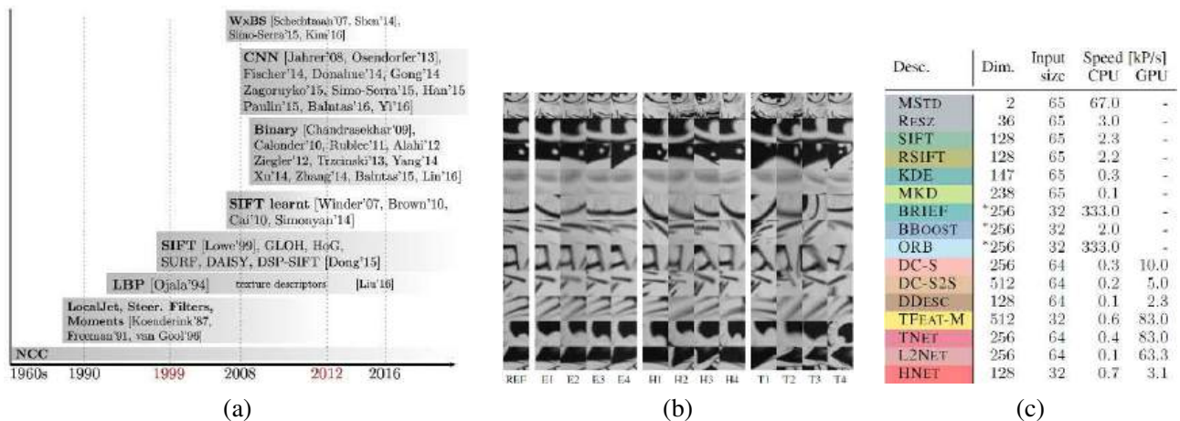
Figure 7.20 Hatches local descriptors benchmark (Balntas, Lenc et al. 2020) © 2019 IEEE: (a) chronology of feature descriptors; (b) typical patches in the dataset (grouped by Easy, Hard, and Tough); (c) size and speed of different descriptors.
