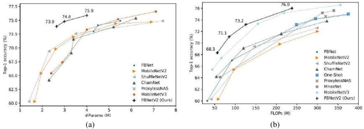
Figure 5.45 ImageNet accuracy vs. (a) size (# of parameters) and (b) operation counts for a number of recent efficient networks (Wan, Dai et al. 2020) © 2020 IEEE.
