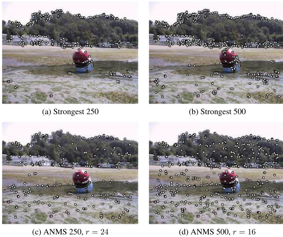
Figure 7.9 Adaptive non-maximal suppression (ANMS) (Brown, Szeliski, and Winder 2005) © 2005 IEEE: The upper two images show the strongest 250 and 500 interest points, while the lower two images show the interest points selected with adaptive non-maximal suppression, along with the corresponding suppression radius r . Note how the latter features have a much more uniform spatial distribution across the image.
