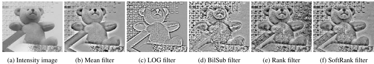
Figure 12.8 Various similarity measures (pre-processing filters) studied in (Hirschmüller and Scharstein 2009) © 2009 IEEE. The contrast of (b)–(d) has been increased for better visualization.
