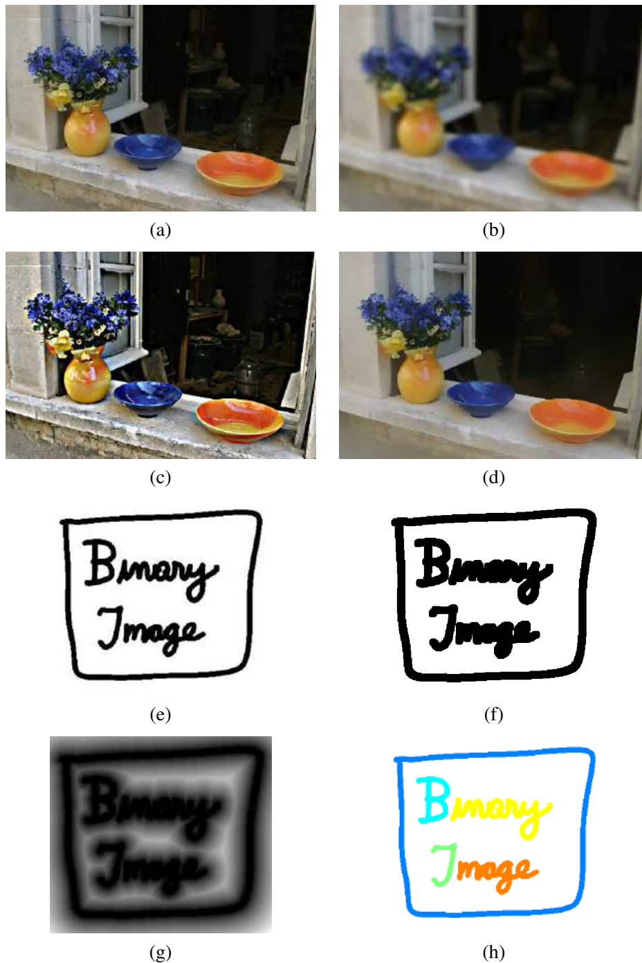
Figure 3.11 Some neighborhood operations: (a) original image; (b) blurred; (c) sharpened; (d) smoothed with edge-preserving filter; (e) binary image; (f) dilated; (g) distance transform; (h) connected components. For the dilation and connected components, black (ink) pixels are assumed to be active, i.e., to have a value of 1 in Equations (3.44–3.48).
