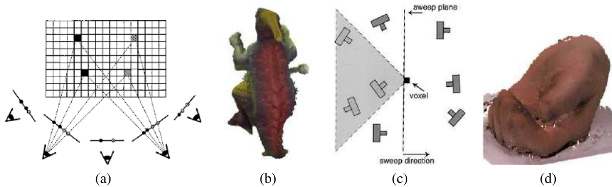
Figure 12.28 Voxel coloring (Seitz and Dyer 1999) © 1999 Springer and space carving (Kutulakos and Seitz 2000) © 2000 Springer. (a–b): voxel coloring sweeps a plane through the scene in a front-to-back manner with respect to the cameras. (c–d): space carving uses multiple sweep directions to deal with more general camera configurations.
