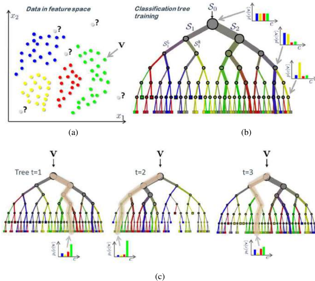
Figure 5.13 Decision trees and forests (Criminisi and Shotton 2013) © 2013 Springer. The top left figure (a) shows a set of training samples tags with four different class colors. The top right (b) shows a single decision tree with a distribution of classes at each node (the root node has the same distribution as the entire training set). During testing (c), each new example (feature vector) is tested at the root node, and depending on this test result (e.g., the comparison of some element to a threshold), a decision is made to walk down the tree to one of its children. This continues until a leaf node with a particular class distribution is reached. During training (b), decisions are selected such that they reduce the entropy (increase class specificity) at the node's children. The bottom diagram (c) shows an ensemble of three trees. After a particular test example has been classified by each tree, the class distributions of the leaf nodes of all the constituent trees are averaged.
