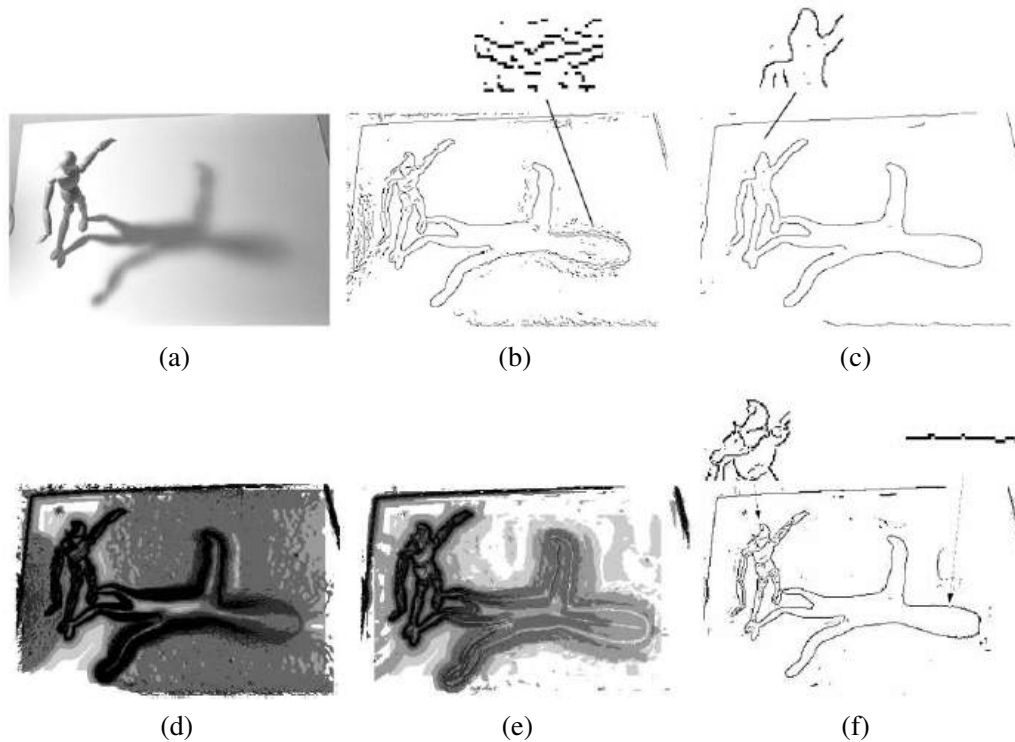
Figure 7.33 Scale selection for edge detection (Elder and Zucker 1998) © 1998 IEEE: (a) original image; (b–c) Canny/Deriche edge detector tuned to the finer (mannequin) and coarser (shadow) scales; (d) minimum reliable scale for gradient estimation; (e) minimum reliable scale for second derivative estimation; (f) final detected edges.
