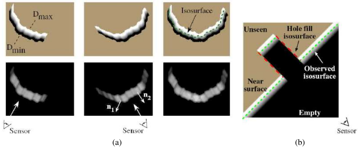
Figure 13.11 Range data merging (Curless and Levoy 1996) © 1996 ACM: (a) two signed distance functions (top left) are merged with their (weights) bottom left to produce a combined set of functions (right column) from which an isosurface can be extracted (green dashed line); (b) the signed distance functions are combined with empty and unseen space labels to fill holes in the isosurface.
