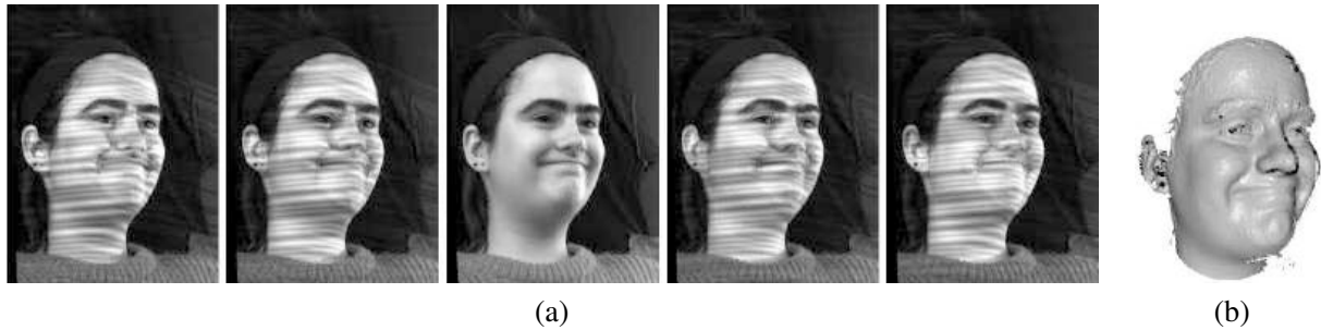
Figure 13.10 Real-time dense 3D face capture using spacetime stereo (Zhang, Snavely et al. 2004) © 2004 ACM: (a) set of five consecutive video frames from one of two stereo cameras (every fifth frame is free of stripe patterns, in order to extract texture); (b) resulting high-quality 3D surface model (depth map visualized as a shaded rendering).
