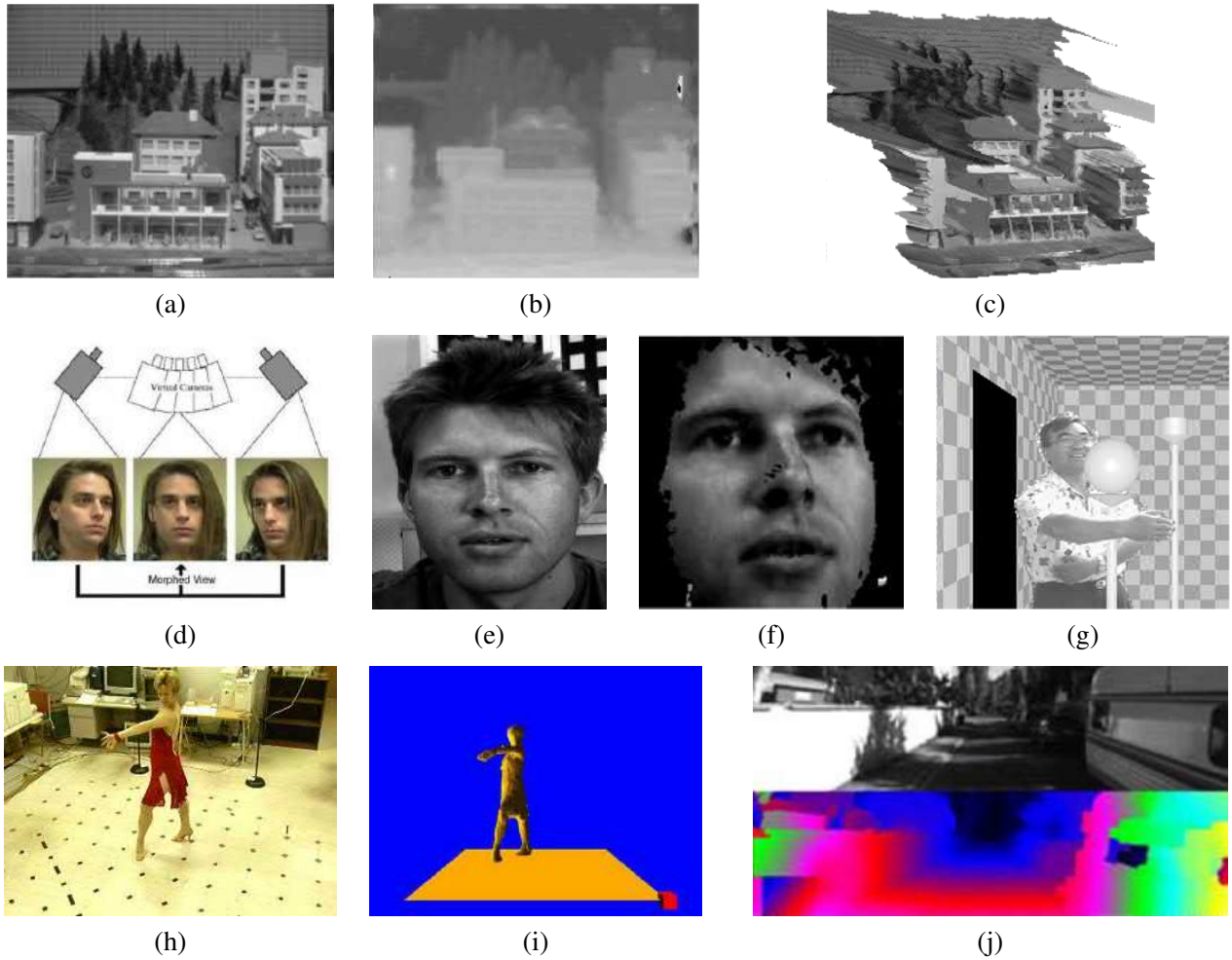
Figure 12.2 Applications of stereo vision: (a) input image, (b) computed depth map, and (c) new view generation from multi-view stereo (Matthies, Kanade, and Szeliski 1989) © 1989 Springer; (d) view morphing between two images (Seitz and Dyer 1996) © 1996 ACM; (e–f) 3D face modeling (images courtesy of Frédéric Devernay); (g) z-keying live and computer-generated imagery (Kanade, Yoshida et al. 1996) © 1996 IEEE; (h–i) building 3D surface models from multiple video streams in Virtualized Reality (Kanade, Rander, and Narayanan 1997) © 1997 IEEE; (j) computing depth maps for autonomous navigation (Geiger, Lenz, and Urtasun 2012) © 2012 IEEE.
