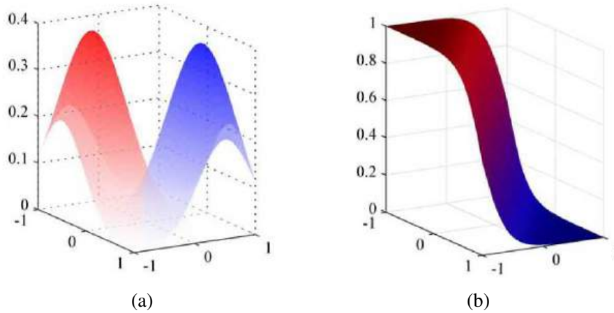
Figure 5.8 Logistic regression for two identically distributed Gaussian classes (Bishop 2006) © 2006 Springer: (a) two Gaussian distributions shown in red and blue; (b) the posterior probability p(C_0|\mathbf{x}) , shown as both the height of the function and the proportion of red ink.
