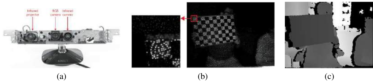
Figure 13.9 The Microsoft Kinect depth camera (Zhang 2012) © 2012 IEEE: (a) the hardware, comprising an infrared (IR) speckle pattern projector and a color and IR camera pair; (b) close-up of a sample infrared image, showing the projected dots; (c) the final depth map, which has black “shadows” in the areas not illuminated by the projector.
