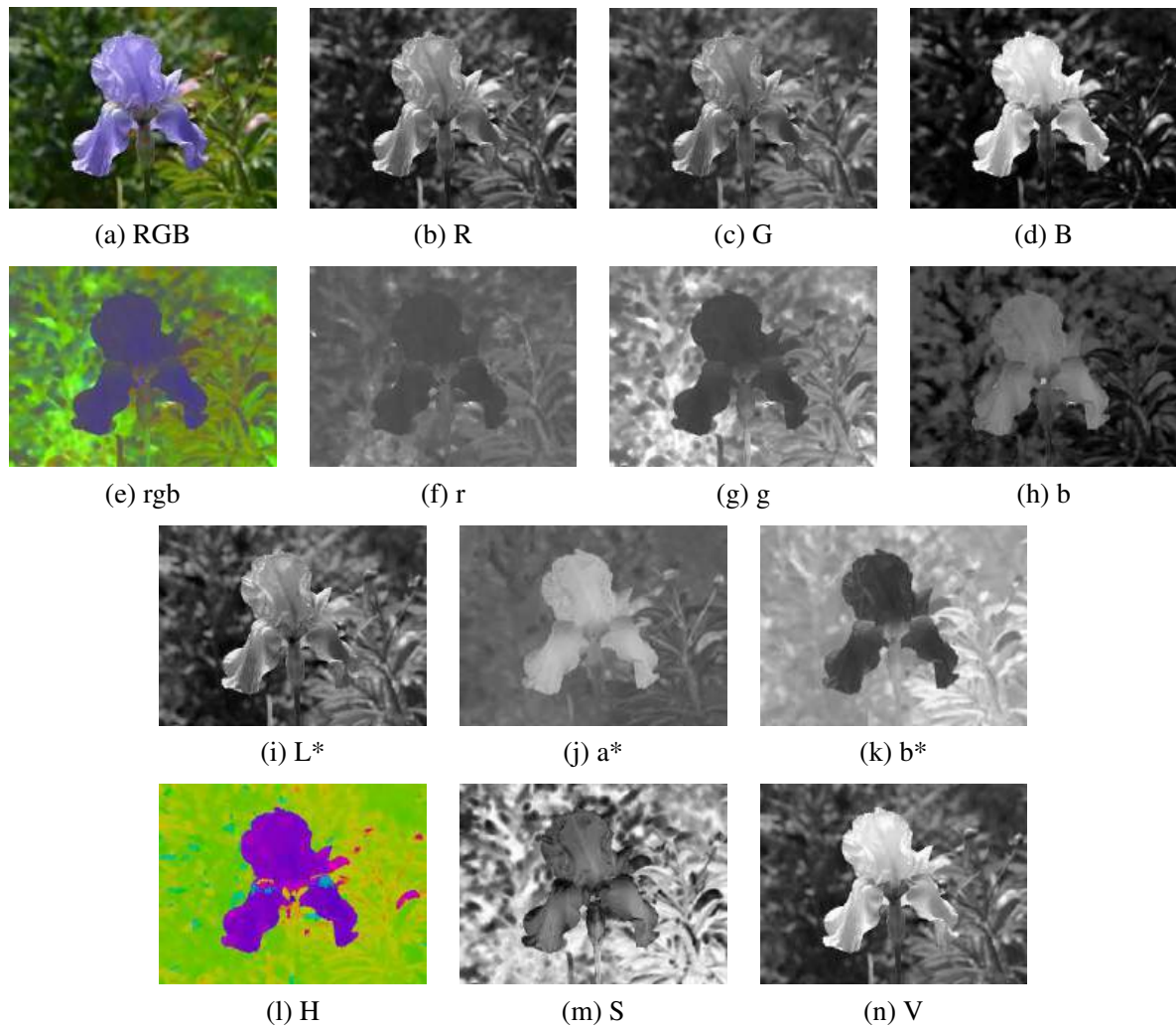
Figure 2.33 Color space transformations: (a–d) RGB; (e–h) rgb. (i–k) L^*a^*b^* ; (l–n) HSV. Note that the rgb, L^*a^*b^* , and HSV values are all re-scaled to fit the dynamic range of the printed page.
