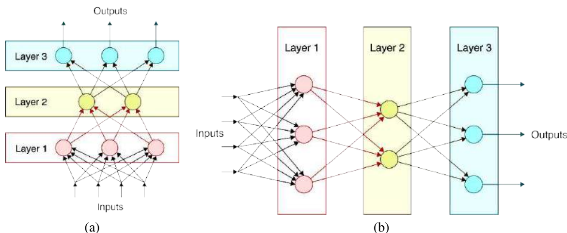
Figure 5.25 Two different ways to draw neural networks: (a) inputs at bottom, outputs at top, (b) inputs at left, outputs at right. © Glassner (2018)
