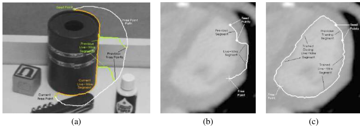
Figure 7.43 Intelligent scissors: (a) as the mouse traces the white path, the scissors follow the orange path along the object boundary (the green curves show intermediate positions) (Mortensen and Barrett 1995) © 1995 ACM; (b) regular scissors can sometimes jump to a stronger (incorrect) boundary; (c) after training to the previous segment, similar edge profiles are preferred (Mortensen and Barrett 1998) © 1995 Elsevier.
