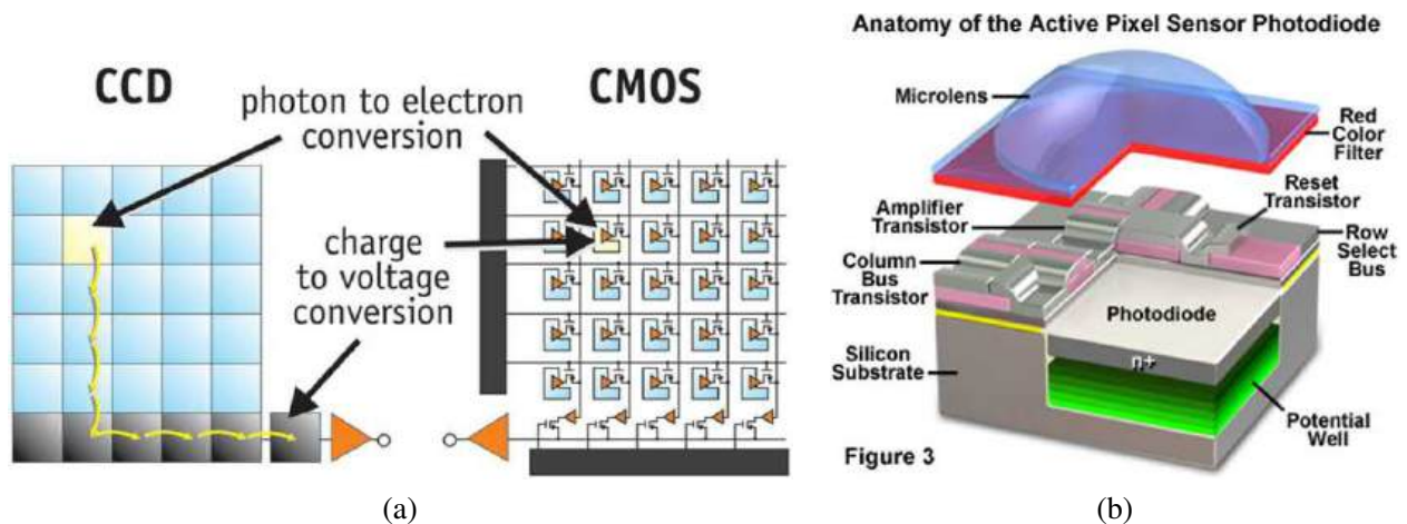
Figure 2.24 Digital imaging sensors: (a) CCDs move photogenerated charge from pixel to pixel and convert it to voltage at the output node; CMOS imagers convert charge to voltage inside each pixel (Litwiller 2005) © 2005 Photonics Spectra; (b) cutaway diagram of a CMOS pixel sensor, from https://micro.magnet.fsu.edu/primer/digitalimaging/cmosimagesensors.html .
