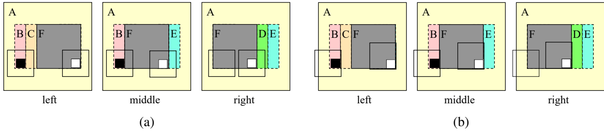
Figure 12.20 Spatio-temporally shiftable windows (Kang, Szeliski, and Chai 2001) © 2001 IEEE: A simple three-image sequence (the middle image is the reference image), which has a moving frontal gray square (marked F) and a stationary background. Regions B, C, D, and E are partially occluded. (a) A regular SSD algorithm will make mistakes when matching pixels in these regions (e.g., the window centered on the black pixel in region B) and in windows straddling depth discontinuities (the window centered on the white pixel in region F). (b) Shiftable windows help mitigate the problems in partially occluded regions and near depth discontinuities. The shifted window centered on the white pixel in region F matches correctly in all frames. The shifted window centered on the black pixel in region B matches correctly in the left image, but requires temporal selection to disable matching the right image. Figure 12.19b shows an EPI corresponding to this sequence and describes in more detail how temporal selection works.
