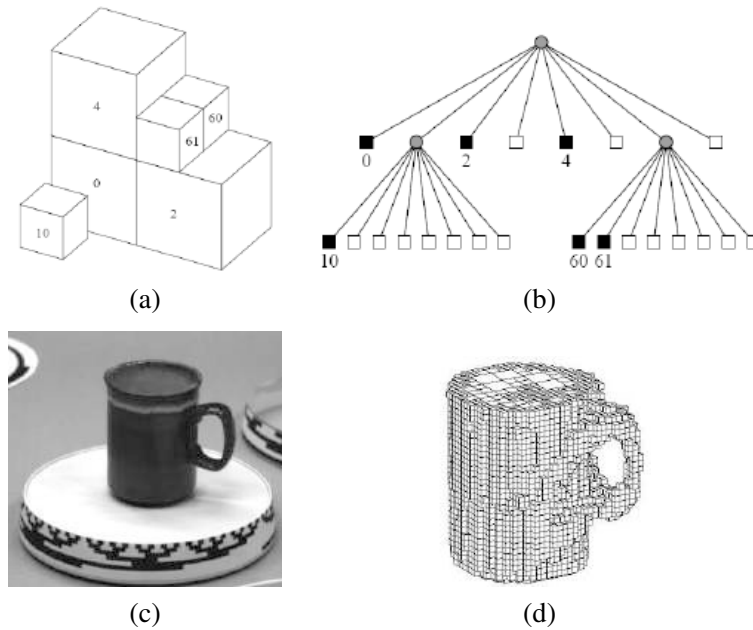
Figure 12.29 Volumetric octree reconstruction from binary silhouettes (Szeliski 1993) © 1993 Elsevier: (a) octree representation and its corresponding (b) tree structure; (c) input image of an object on a turntable; (d) computed 3D volumetric octree model.
