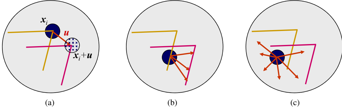
Figure 7.4 Aperture problems for different image patches: (a) stable (“corner-like”) flow; (b) classic aperture problem (barber-pole illusion); (c) textureless region. The two images I_0 (yellow) and I_1 (red) are overlaid. The red vector \mathbf{u} indicates the displacement between the patch centers and the w(\mathbf{x}_i) weighting function (patch window) is shown as a dark circle.
