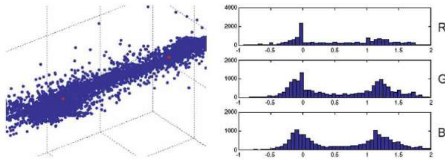
Figure 10.37 Two-color model computed from a collection of local 5 \times 5 neighborhoods (Bennett, Uyttendaele et al. 2006) © 2006 Springer. After two-means clustering and reprojection along the line joining the two dominant colors (red dots), the majority of the pixels fall near the fitted line. The distribution along the line, projected along the RGB axes, is peaked at 0 and 1, the two dominant colors.
