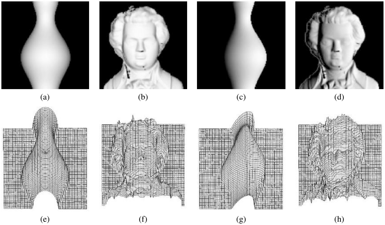
Figure 13.2 Synthetic shape from shading (Zhang, Tsai et al. 1999) © 1999 IEEE: shaded images, (a–b) with light from in front (0, 0, 1) and (c–d) with light from the front right (1, 0, 1); (e–f) corresponding shape from shading reconstructions using the technique of Tsai and Shah (1994).
