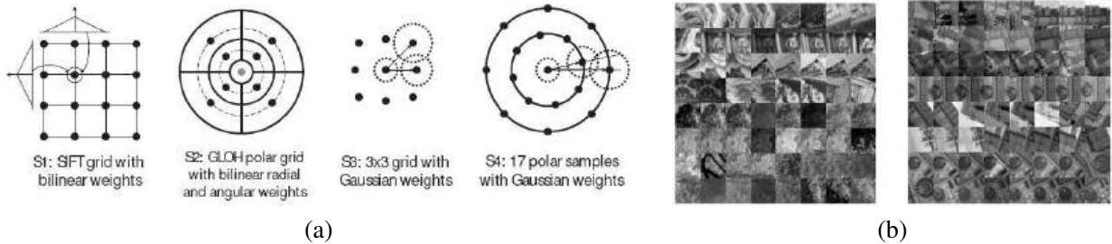
Figure 7.18 Spatial summation blocks for SIFT, GLOH, and some related feature descriptors (Winder and Brown 2007) © 2007 IEEE: (a) The parameters for the features, e.g., their Gaussian weights, are learned from a training database of (b) matched real-world image patches obtained from robust structure from motion applied to internet photo collections (Hua, Brown, and Winder 2007).
