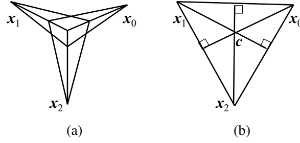
Figure 11.3 Calibration from vanishing points: (a) any pair of finite vanishing points ( \hat{\mathbf{x}}_i, \hat{\mathbf{x}}_j ) can be used to estimate the focal length; (b) the orthocenter of the vanishing point triangle gives the image center of the image \mathbf{c} .
