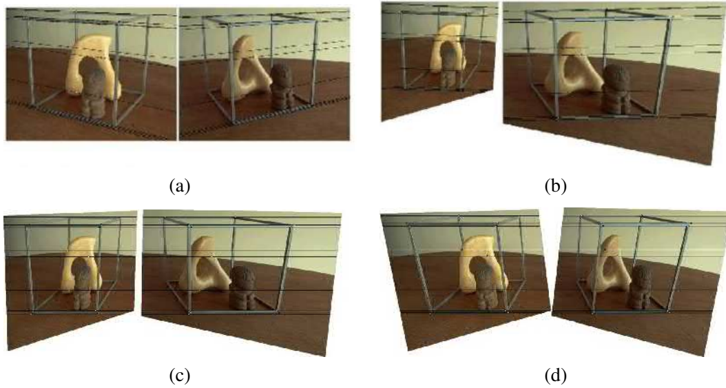
Figure 12.4 The multi-stage stereo rectification algorithm of Loop and Zhang (1999) © 1999 IEEE. (a) Original image pair overlaid with several epipolar lines; (b) images transformed so that epipolar lines are parallel; (c) images rectified so that epipolar lines are horizontal and in vertical correspondence; (d) final rectification that minimizes horizontal distortions.
