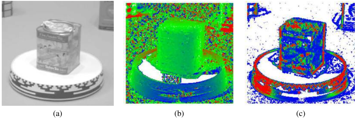
Figure 12.11 Uncertainty in stereo depth estimation (Szeliski 1991b): (a) input image; (b) estimated depth map (blue is closer); (c) estimated confidence (red is higher). As you can see, more textured areas have higher confidence.
