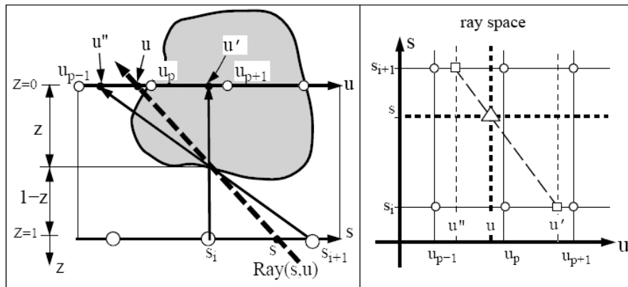
Figure 14.12 Depth compensation in the Lumigraph (Gortler, Grzeszczuk et al. 1996) © 1996 ACM. To re-sample the (s, u) dashed light ray, the u parameter corresponding to each discrete s_i camera location is modified according to the out-of-plane depth z to yield new coordinates u and u' ; in (u, s) ray space, the original sample ( \triangle ) is resampled from the (s_i, u') and (s_{i+1}, u'') samples, which are themselves linear blends of their adjacent ( \circ ) samples.
