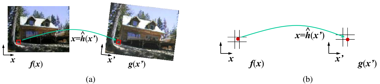
Figure 3.46 Inverse warping algorithm: (a) a pixel g(x') is sampled from its corresponding location x = \hat{h}(x') in image f(x) ; (b) detail of the source and destination pixel locations.
