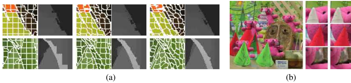
Figure 12.15 Stereo matching with adaptive over-segmentation and matting (Taguchi, Wilburn, and Zitnick 2008) © 2008 IEEE: (a) segment boundaries are refined during the optimization, leading to more accurate results (e.g., the thin green leaf in the bottom row); (b) alpha mattes are extracted at segment boundaries, which leads to visually better compositing results (middle column).
