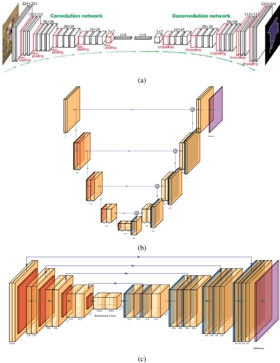
Figure 5.37 (a) The deconvolution network of Noh, Hong, and Han (2015) © 2015 IEEE and (b–c) the U-Net of Ronneberger, Fischer, and Brox (2015), drawn using the PlotNeuralNet LaTeX package. In addition to the fine-to-coarse-to-fine bottleneck used in (a), the U-Net also has skip connections between encoding and decoding layers at the same resolution.
