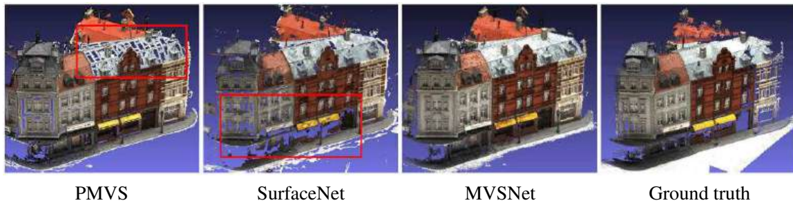
Figure 12.22 Depth maps computed using three different multi-view stereo algorithms shown as colored point clouds (Yao, Luo et al. 2018) © 2018 Springer. The red boxes indicate problem areas where MVSNet does better.
