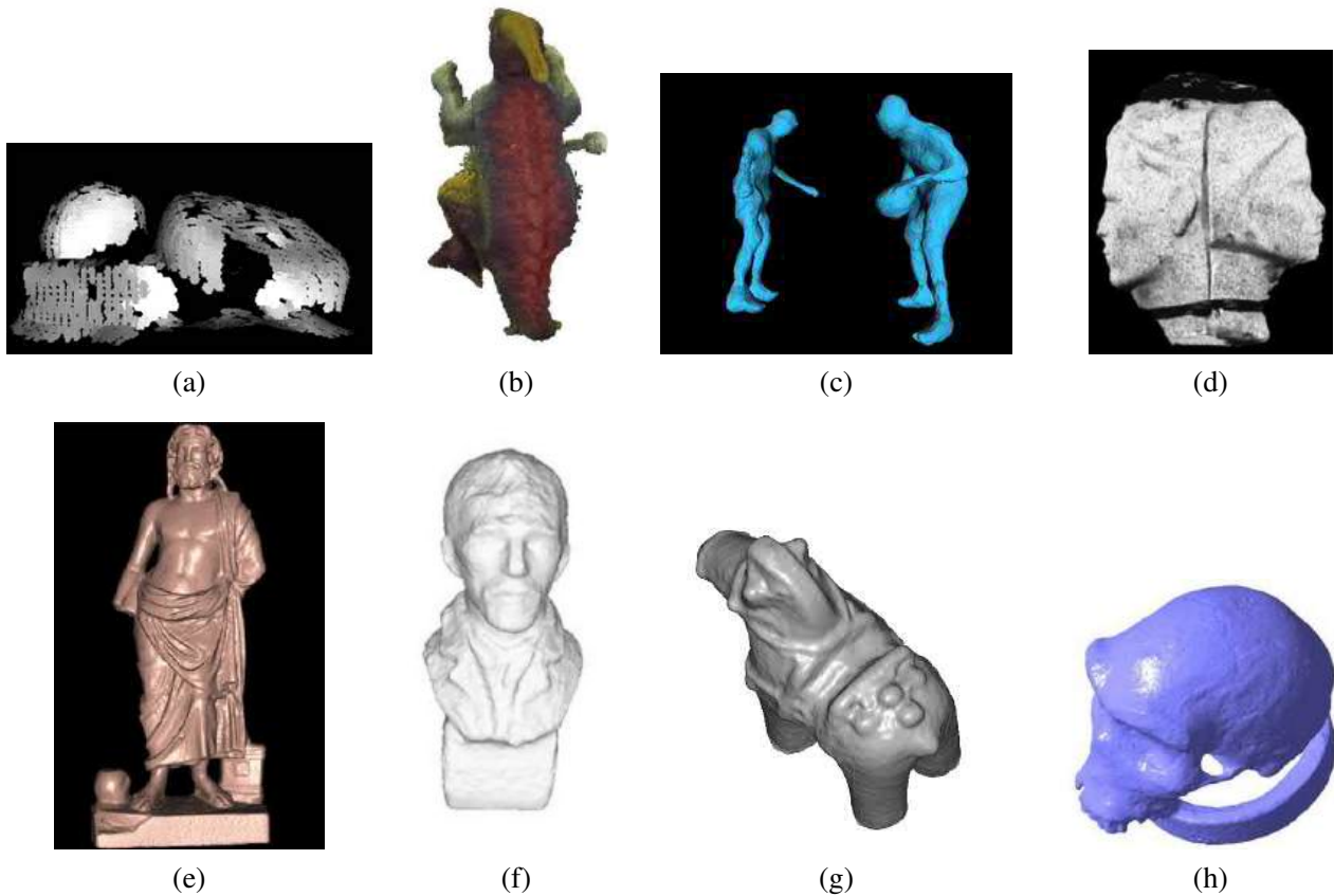
Figure 12.24 Multi-view stereo algorithms: (a) surface-based stereo (Fua and Leclerc 1995) © 1995 Springer; (b) voxel coloring (Seitz and Dyer 1999) © 1999 Springer; (c) depth map merging (Narayanan, Rander, and Kanade 1998) © 1998 IEEE; (d) level set evolution (Faugeras and Keriven 1998) © 1998 IEEE; (e) silhouette and stereo fusion (Hernández and Schmitt 2004) © 2004 Elsevier; (f) multi-view image matching (Pons, Keriven, and Faugeras 2005) © 2005 IEEE; (g) volumetric graph cut (Vogiatzis, Torr, and Cipolla 2005) © 2005 IEEE; (h) carved visual hulls (Furukawa and Ponce 2009) © 2009 Springer.
