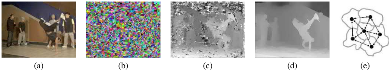
Figure 12.14 Segmentation-based stereo matching (Zitnick, Kang et al. 2004) © 2004 ACM: (a) input color image; (b) color-based segmentation; (c) initial disparity estimates; (d) final piecewise-smoothed disparities; (e) MRF neighborhood defined over the segments in the disparity space distribution (Zitnick and Kang 2007) © 2007 Springer.
