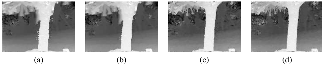
Figure 12.21 Local ( 5 \times 5 window-based) matching results (Kang, Szeliski, and Chai 2001) © 2001 IEEE: (a) window that is not spatially perturbed (centered); (b) spatially perturbed window; (c) using the best five of 10 neighboring frames; (d) using the better half sequence. Notice how the results near the tree trunk are improved using temporal selection.
