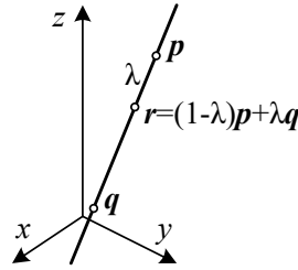
Figure 2.3 3D line equation, \mathbf{r} = (1 - \lambda)\mathbf{p} + \lambda\mathbf{q} .
