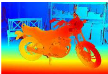
12. Depth estimation
