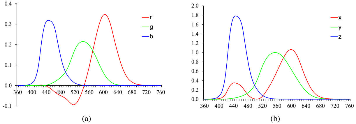
Figure 2.29 Standard CIE color matching functions: (a) \bar{r}(\lambda) , \bar{g}(\lambda) , \bar{b}(\lambda) color spectra obtained from matching pure colors to the R=700.0nm, G=546.1nm, and B=435.8nm primaries; (b) \bar{x}(\lambda) , \bar{y}(\lambda) , \bar{z}(\lambda) color matching functions, which are linear combinations of the (\bar{r}(\lambda), \bar{g}(\lambda), \bar{b}(\lambda)) spectra.
