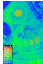
10. Computational Photography
