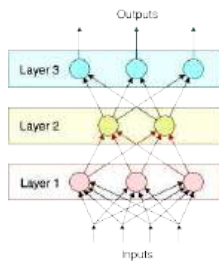
5. Deep learning
