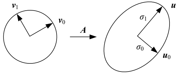
Figure A.1 The action of a matrix \mathbf{A} can be visualized by thinking of the domain as being spanned by a set of orthonormal vectors \mathbf{v}_j , each of which is transformed to a new orthogonal vector \mathbf{u}_j with a length \sigma_j . When \mathbf{A} is interpreted as a covariance matrix and its eigenvalue decomposition is performed, each of the \mathbf{u}_j axes denote a principal direction (component) and each \sigma_j denotes one standard deviation along that direction.
