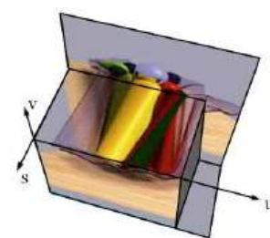
14. Image-based Rendering
