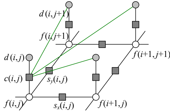
Figure 4.18 Graphical model for a discriminative random field (DRF). The additional green edges show how combinations of sensed data, e.g., d(i, j+1) , influence the data term for f(i, j) . The generative model is therefore more complex, i.e., we cannot just apply a simple function to the unknown variables and add noise.
