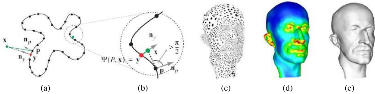
Figure 13.17 Point-based surface modeling with moving least squares (MLS) (Pauly, Keiser et al. 2003) © 2003 ACM: (a) a set of points (black dots) is turned into an implicit inside–outside function (black curve); (b) the signed distance to the nearest oriented point can serve as an approximation to the inside–outside distance; (c) a set of oriented points with variable sampling density representing a 3D surface (head model); (d) local estimate of sampling density, which is used in the moving least squares; (e) reconstructed continuous 3D surface.
