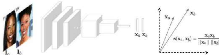
Figure 6.18 A typical modern deep face recognition architecture, from the survey by Masi, Wu et al. (2018) © 2018 IEEE. At training time, a huge labeled face set (a) is used to constrain the weights of a DCNN (b), optimizing a loss function (c) for a classification task. At test time, the classification layer is often discarded, and the DCNN is used as a feature extractor for comparing face descriptors.
