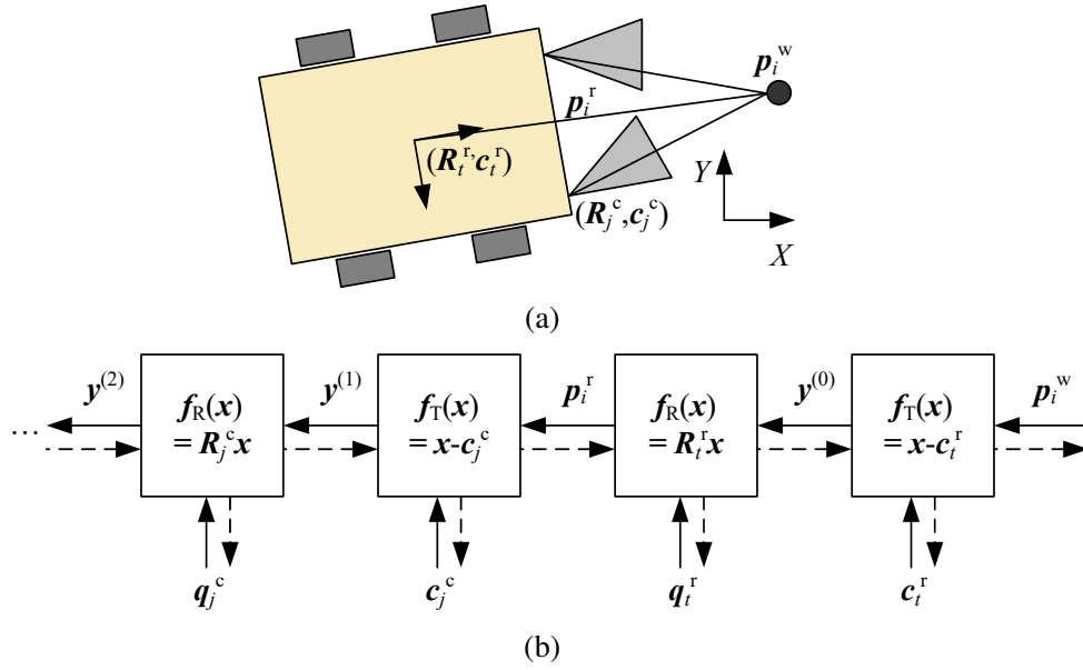
Figure 11.15 A camera rig and its associated transform chain. (a) As the mobile rig (robot) moves around in the world, its pose with respect to the world at time t is captured by (R_t^r, c_t^r) . Each camera's pose with respect to the rig is captured by (R_j^c, c_j^c) . (b) A 3D point with world coordinates p_i^w is first transformed into rig coordinates p_i^r , and then through the rest of the camera-specific chain, as shown in Figure 11.14.
