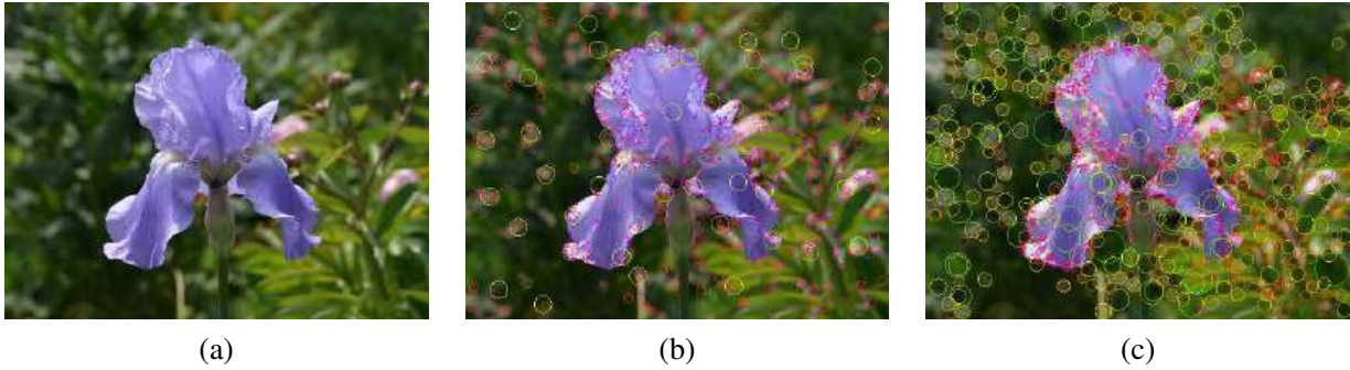
Figure 7.8 Interest operator responses: (a) Sample image, (b) Harris response, and (c) DoG response. The circle sizes and colors indicate the scale at which each interest point was detected. Notice how the two detectors tend to respond at complementary locations.
