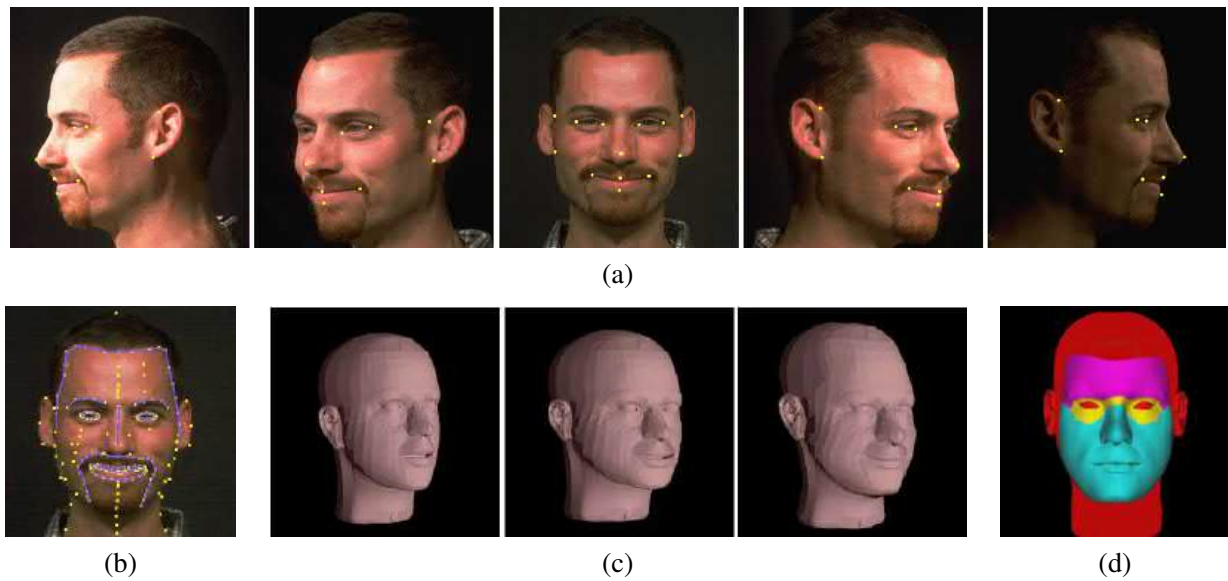
Figure 13.22 3D model fitting to a collection of images: (Pighin, Hecker et al. 1998) © 1998 ACM: (a) set of five input images along with user-selected keypoints; (b) the complete set of keypoints and curves; (c) three meshes—the original, adapted after 13 keypoints, and after an additional 99 keypoints; (d) the partition of the image into separately animatable regions.
