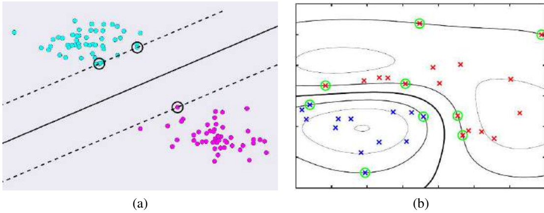
Figure 5.11 (a) A support vector machine (SVM) finds the linear decision surface (hyper-plane) that maximizes the margin to the nearest training examples, which are called the support vectors © Glassner (2018). (b) A two-dimensional two class example of a Gaussian kernel support vector machine (Bishop 2006) © 2006 Springer. The red and blue \times s indicate the training samples, and the samples circled in green are the support vectors. The black lines indicate iso-contours of the kernel regression function, with the contours containing the blue and red support vectors indicating the \pm 1 contours and the dark contour in between being the decision surface.
