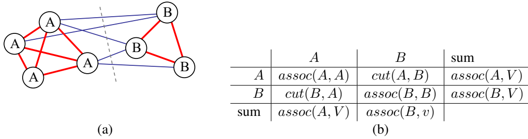
Figure 7.54 Sample weighted graph and its normalized cut: (a) a small sample graph and its smallest normalized cut; (b) tabular form of the associations and cuts for this graph. The assoc and cut entries are computed as area sums of the associated weight matrix \mathbf{W} . Normalizing the table entries by the row or column sums produces normalized associations and cuts N_{assoc} and N_{cut} .
