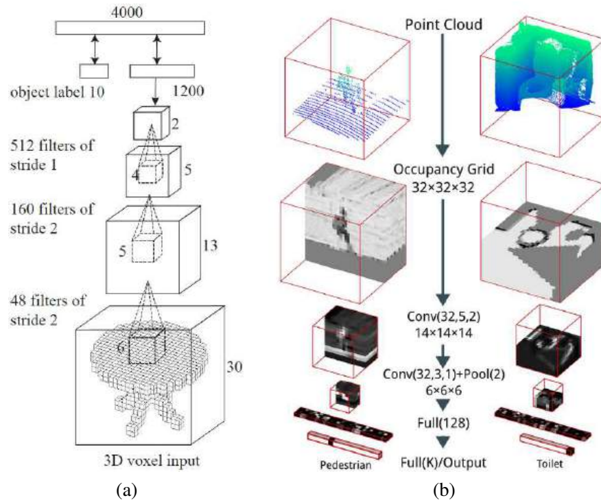
Figure 5.53 3D convolutional networks applied to volumetric data for object detection: (a) 3D ShapeNets (Wu, Song et al. 2015) © 2015 IEEE; (b) VoxNet (Maturana and Scherer 2015) © 2015 IEEE.
