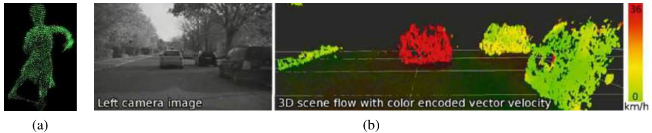
Figure 12.23 Three-dimensional scene flow: (a) computed from a multi-camera dome surrounding the dancer shown in Figure 12.2h–j (Vedula, Baker et al. 2005) © 2005 IEEE; (b) computed from stereo cameras mounted on a moving vehicle (Wedel, Rabe et al. 2008) © 2008 Springer.
