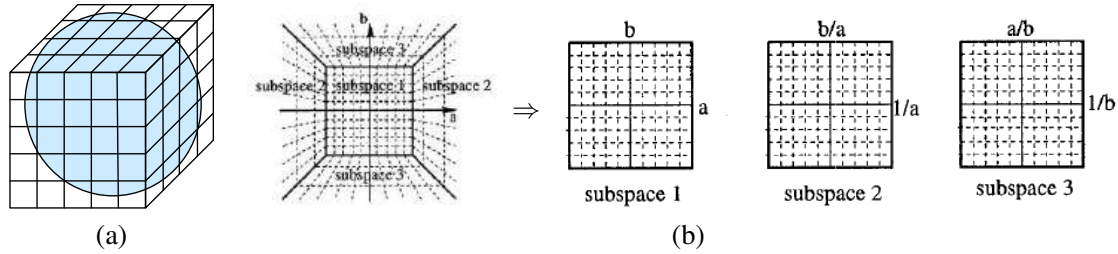
Figure 7.49 Cube map representation for line equations and vanishing points: (a) a cube map surrounding the unit sphere; (b) projecting the half-cube onto three subspaces (Tuytelaars, Van Gool, and Proesmans 1997) © 1997 IEEE.
