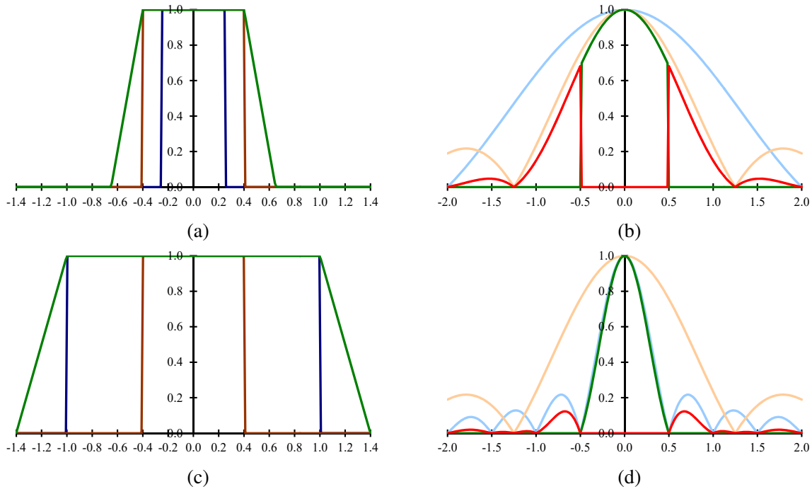
Figure 2.27 Sample point spread functions (PSF): The diameter of the blur disc (blue) in (a) is equal to half the pixel spacing, while the diameter in (c) is twice the pixel spacing. The horizontal fill factor of the sensing chip is 80% and is shown in brown. The convolution of these two kernels gives the point spread function, shown in green. The Fourier response of the PSF (the MTF) is plotted in (b) and (d). The area above the Nyquist frequency where aliasing occurs is shown in red.
