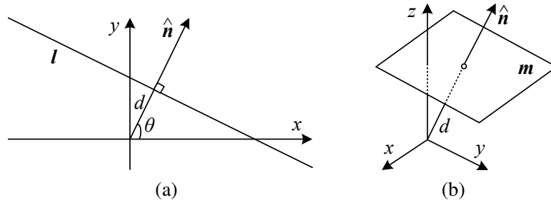
Figure 2.2 (a) 2D line equation and (b) 3D plane equation, expressed in terms of the normal \hat{\mathbf{n}} and distance to the origin d .
