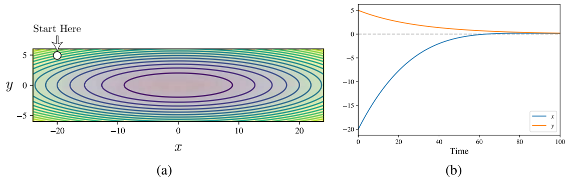
Figure 5.63 Function optimization: (a) the contour plot of f(x, y) = x^2 + 20y^2 with the function being minimized at (0, 0) ; (b) ideal gradient descent optimization that quickly converges towards the minimum at x = 0 , y = 0 .
