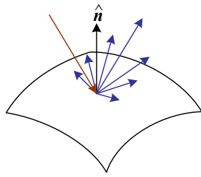
2. Image formation
