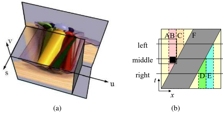
Figure 12.19 Epipolar plane image (EPI) (Gortler, Grzeszczuk et al. 1996) © 1996 ACM and a schematic EPI (Kang, Szeliski, and Chai 2001) © 2001 IEEE. (a) The Lumigraph (light field) (Section 14.3) is the 4D space of all light rays passing through a volume of space. Taking a 2D slice results in all of the light rays embedded in a plane and is equivalent to a scanline taken from a stacked EPI volume. Objects at different depths move sideways with velocities (slopes) proportional to their inverse depth. Occlusion (and translucency) effects can easily be seen in this representation. (b) The EPI corresponding to Figure 12.20 showing the three images (middle, left, and right) as slices through the EPI volume. The spatially and temporally shifted window around the black pixel is indicated by the rectangle, showing that the right image is not being used in matching.
