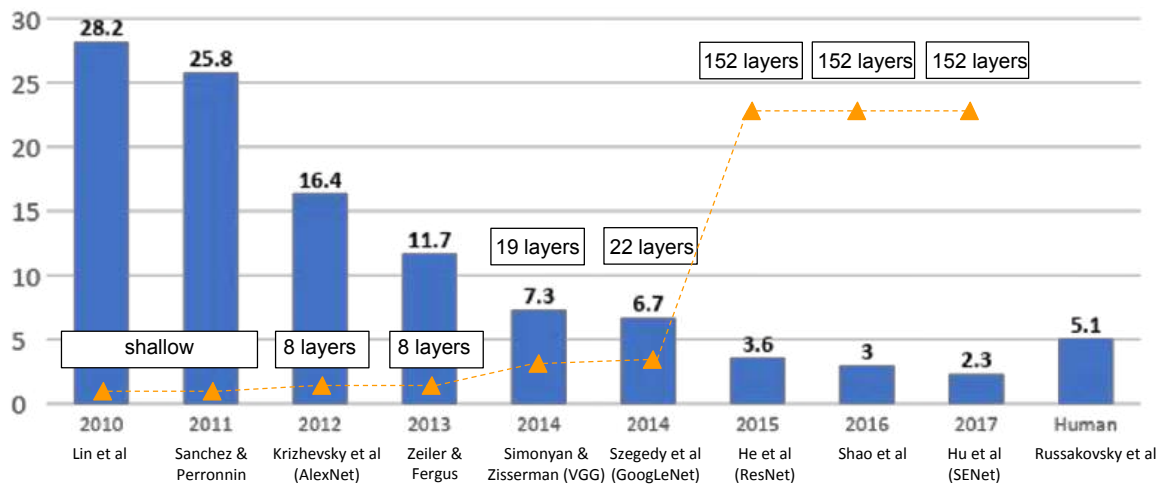
Figure 5.40 Top-5 error rate and network depths of winning entries from the ImageNet Large Scale Visual Recognition Challenge (ILSVRC) © Li, Johnson, and Yeung (2019).
