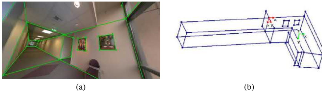
Figure 13.20 Interactive 3D modeling from panoramas (Shum, Han, and Szeliski 1998) © 1998 IEEE: (a) wide-angle view of a panorama with user-drawn vertical and horizontal (axis-aligned) lines; (b) single-view reconstruction of the corridors.
