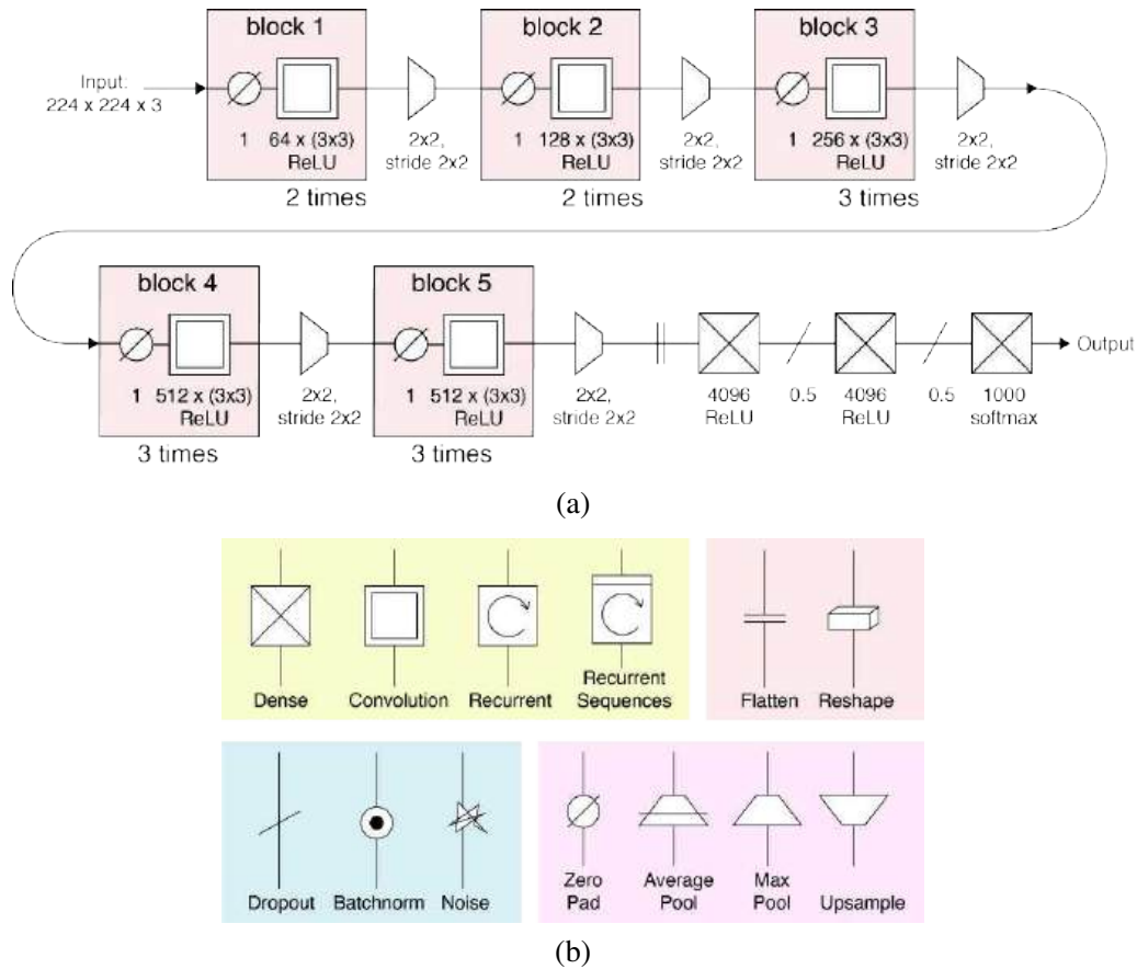
Figure 5.41 The VGG16 network of Simonyan and Zisserman (2014b) © Glassner (2018). (a) The network consists of repeated zero-pad, 3 \times 3 convolution, ReLU blocks interspersed with 2 \times 2 max pooling and a doubling in the number of channels. This is followed by some fully connected and dropout layers, with a final softmax into the 1,000 ImageNet categories. (b) Some of the schematic neural network symbols used by Glassner (2018).
