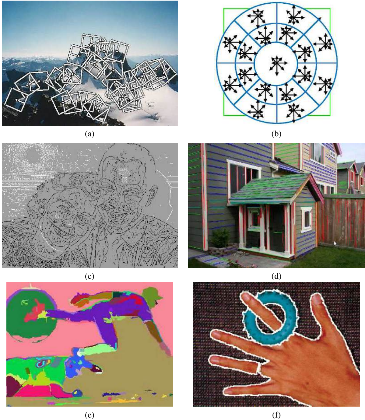
Figure 7.1 Feature detectors and descriptors can be used to analyze, describe and match images: (a) point-like interest operators (Brown, Szeliski, and Winder 2005) © 2005 IEEE; (b) GLOH descriptor (Mikolajczyk and Schmid 2005); (c) edges (Elder and Goldberg 2001) © 2001 IEEE; (d) straight lines (Sinha, Steedly et al. 2008) © 2008 ACM; (e) graph-based merging (Felzenszwalb and Huttenlocher 2004) © 2004 Springer; (f) mean shift (Comaniciu and Meer 2002) © 2002 IEEE.
