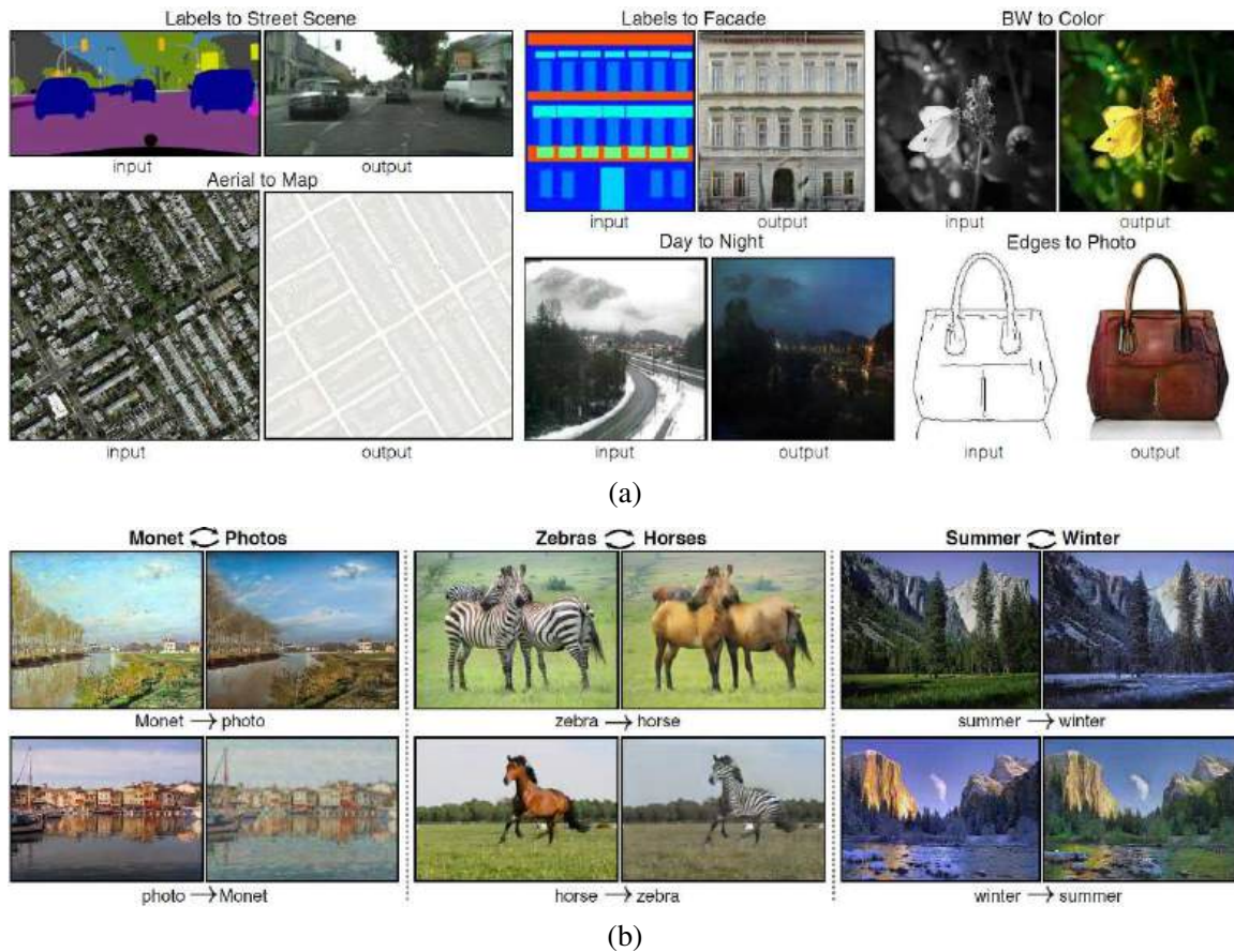
Figure 5.60 Image-to-image translation. (a) Given paired training images, the original pix2pix system learns how to turn sketches into photos, semantic maps to images, and other pixel remapping tasks (Isola, Zhu et al. 2017) © 2017 IEEE. (b) CycleGAN does not require paired training images, just collections coming from different sources, such as painting and photographs or horses and zebras (Zhu, Park et al. 2017) © 2017 IEEE.
