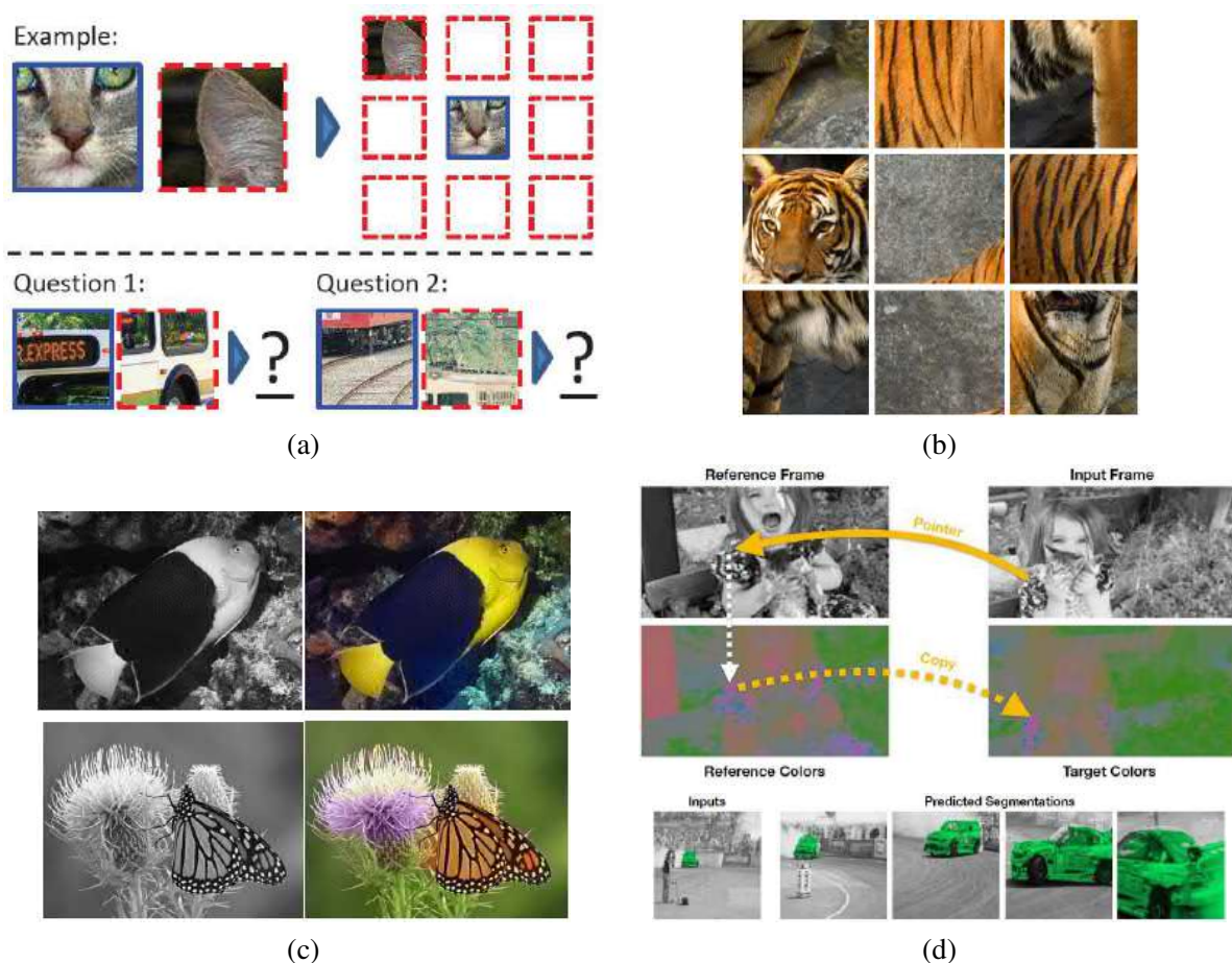
Figure 5.51 Examples of self-supervised learning tasks: (a) guessing the relative positions of image patches—can you guess the answers to Q1 and Q2? (Doersch, Gupta, and Efros 2015) © 2015 IEEE; (b) solving a nine-tile jigsaw puzzle (Noroozi and Favaro 2016) © 2016 Springer; (c) image colorization (Zhang, Isola, and Efros 2016) © 2016 Springer; (d) video color transfer for tracking (Vondrick, Shrivastava et al. 2018) © 2016 Springer.
