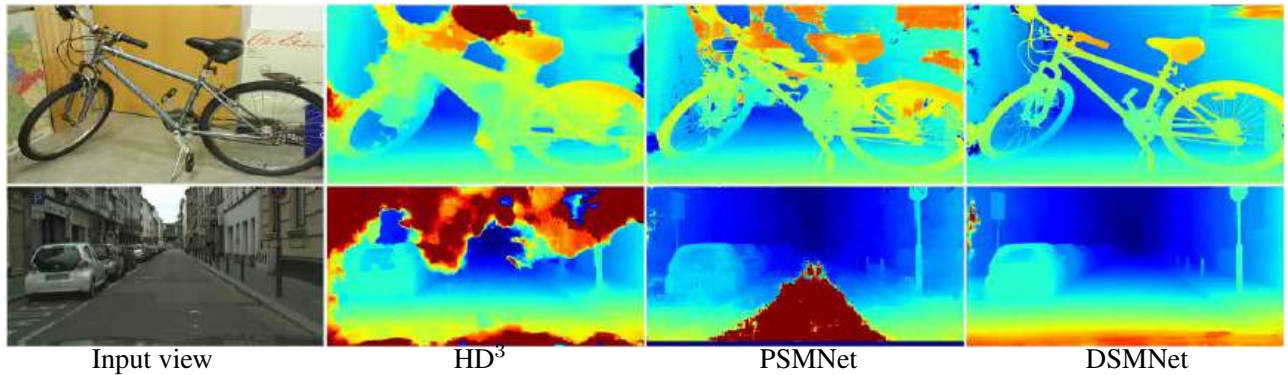
Figure 12.18 Disparity maps computed by three different DNN stereo matchers trained on synthetic data and applied to real-world image pairs (Zhang, Qi et al. 2020) © 2020 Springer.
